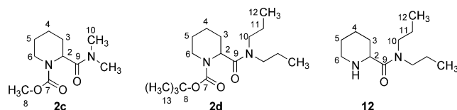
Figure 5. Numbering of carbon atoms of pipecolamides.
