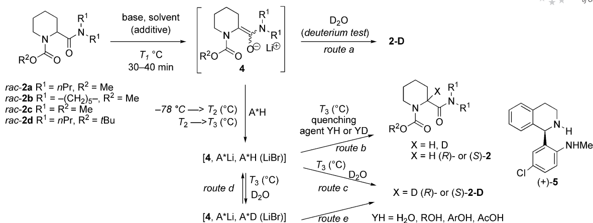
Scheme 1. Deracemization of peicolamides 2 .
