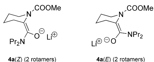
Figure 2. Enolate intermediates 4a .
