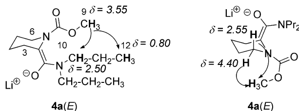
Figure 3. Cross-couplings observed in NMR of enolates 4a ( E ).
