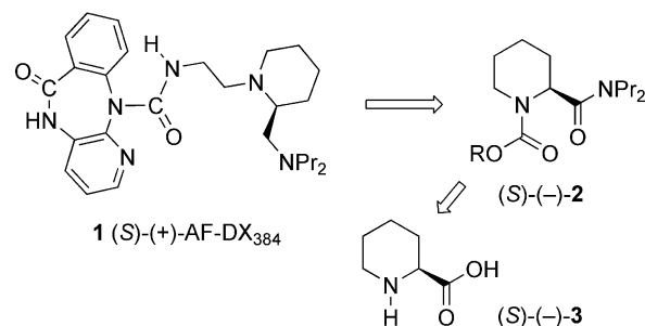
Figure 1. ( S )-(+)-AF-DX 384 from ( S )-(–)-pipecolic acid ( 3 ).
