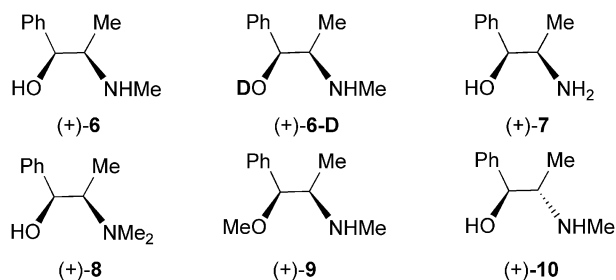
Figure 4. Ephedrine derivatives as chiral sources.
